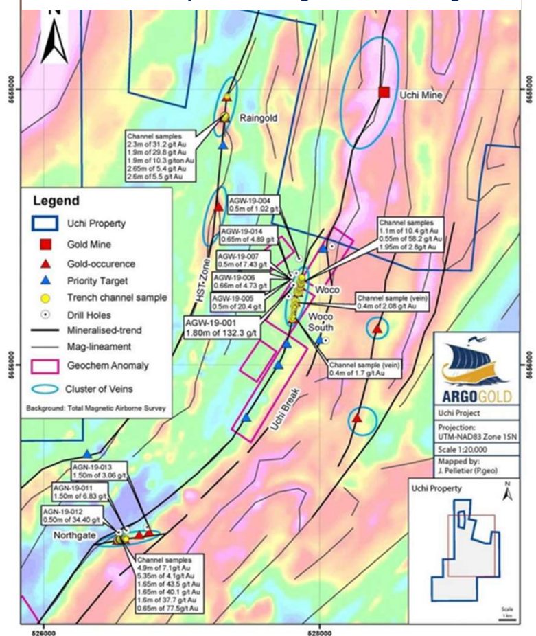
Uchi – Current Exploration Targets on Total Mag
