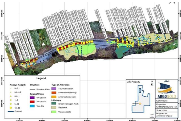
Northgate – Au intersections from channel sampling
